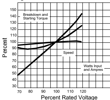
Voltage Variation Effects
