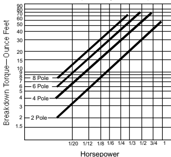
Breakdown Torques by Horsepower
