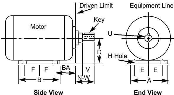
Side View End View Standard NEMA motor frame dimensions.
